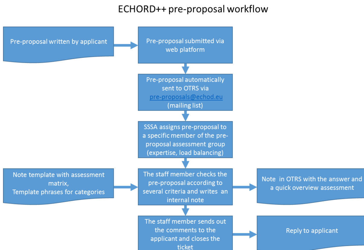
Figure 3: Pre-Proposal Workflow
